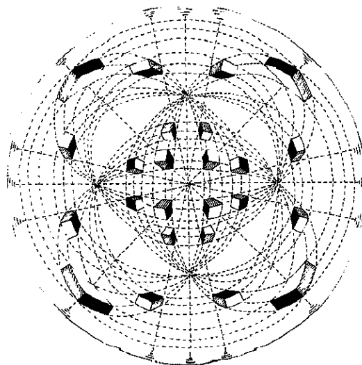
Fig. 6. Twenty-four cubes in Flat-Sphere Perspective.
