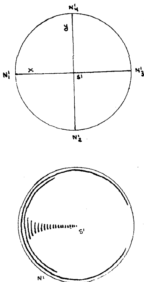
Fig. 8. Two inappropriate representations of schema lines. (Top) The x and y axes appearing without stretching. (Bottom) Simplified representation of the actual stretching that a S - N line on a sphere undergoes when physically flattened on a plane.
