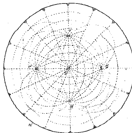
Fig. 5. Symmetrical representation of the Flat-Sphere Perspective schema.
